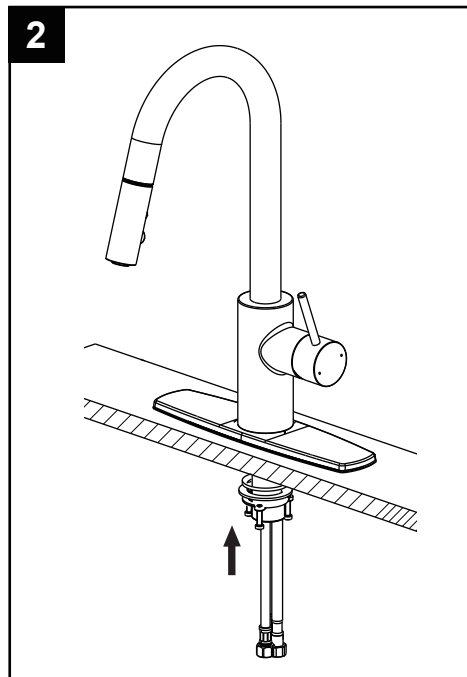
2 Install washer, gasket and mounting nuts onto the shank to cover the mounting hole. Tighten the mounting nut.
